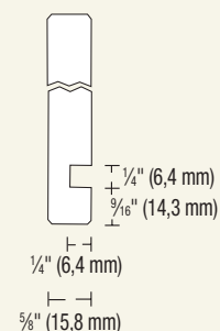
Encoche de fond de tiroir Drawer bottom's notch
