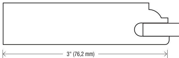
Battant/Rail 03
